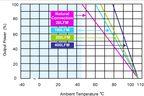
MKW150-24S05, MKW150-24S24, MKW150-48S05, MKW150-48S24 Derating Curve without Heatsink
