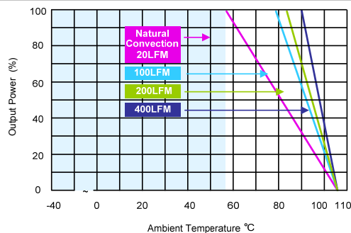
MKW150-24S05, MKW150-24S24, MKW150-48S05, MKW150-48S24 Derating Curve with Heatsink
