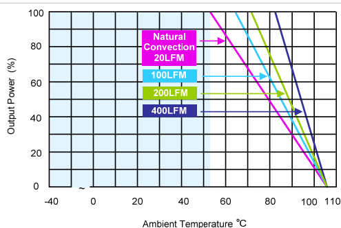
MKW150-24S12, MKW150-24S15, MKW150-48S12, MKW150-48S15 Derating Curve without Heatsink
