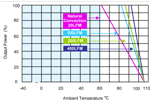
MKW150-24S12, MKW150-24S15, MKW150-48S12, MKW150-48S15 Derating Curve with Heatsink
