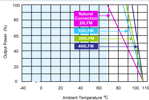
MKW150-24S033, MKW150-48S033 Derating Curve with Heatsink
