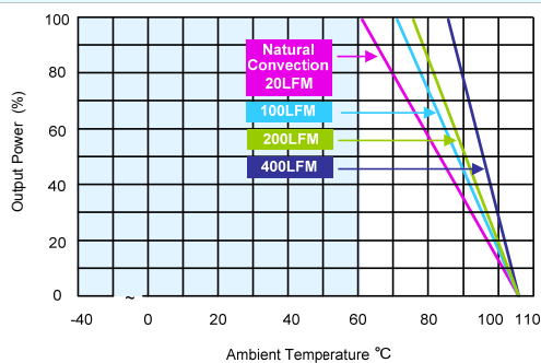
MKW150-24S033, MKW150-48S033 Derating Curve without Heatsink
