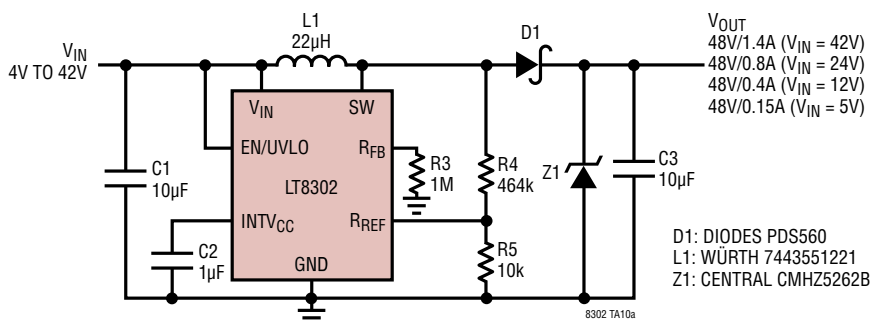
4V to 42V IN /48V OUT Boost Converter
