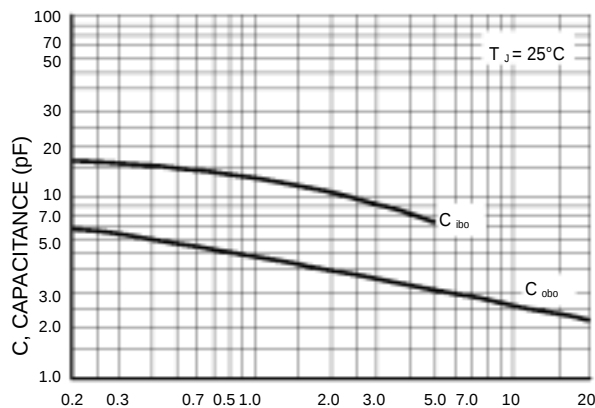
Figure 7. Capacitances
