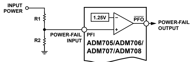
Figure 15. Power-Fail Comparator
