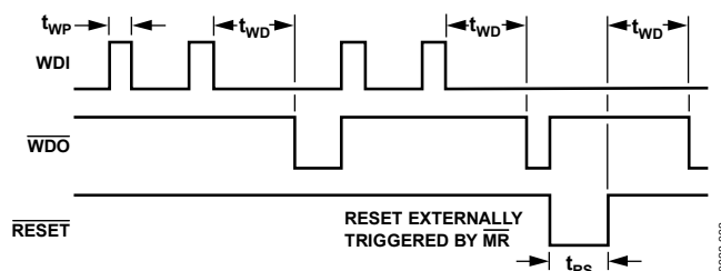
Figure 14. Watchdog Timing
