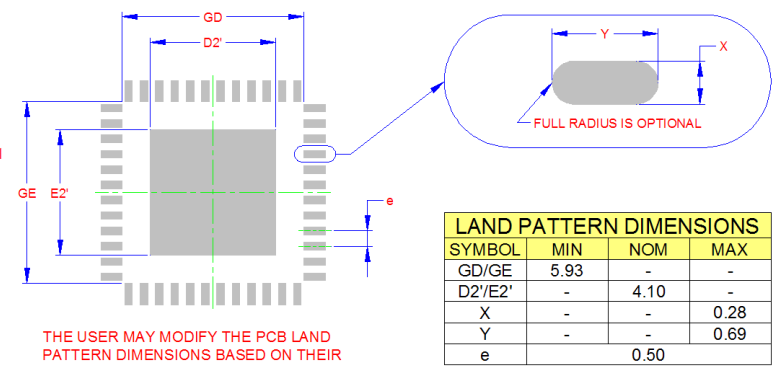
RECOMMENDED PCB LAND PATTERN
