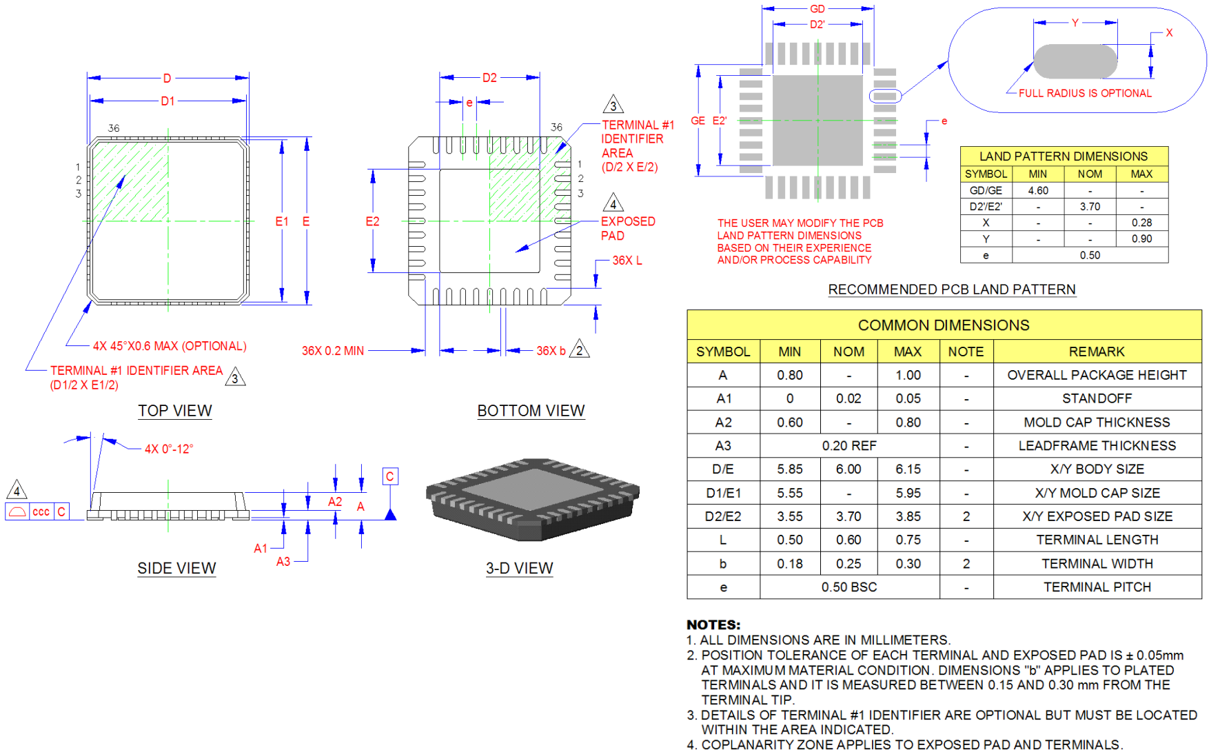
Figure 11.1 36-Pin QFN, 6x6 mm Body, 0.5 mm Pitch
