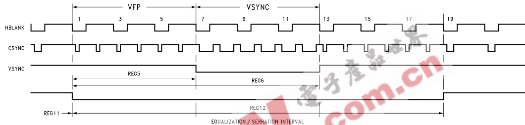
FIGURE 3. Equalization/Serration Interval Programming
