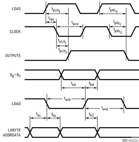
FIGURE 5. AC Specifications
