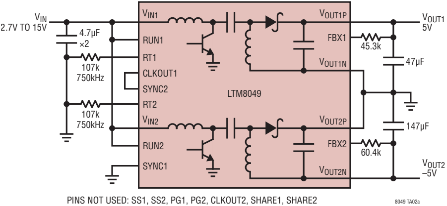
±5V Converter
