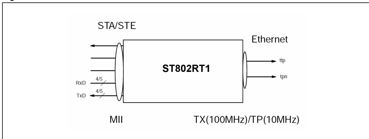
Figure 7. Transmit isolation
