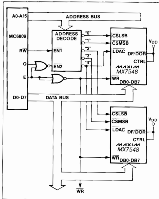
Figure 10. MX7548-MC6809 Interface (Strobed Transfer Mode)
