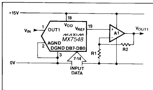
Figure 8. Single Supply Operation Using Voltage Switching Mode
