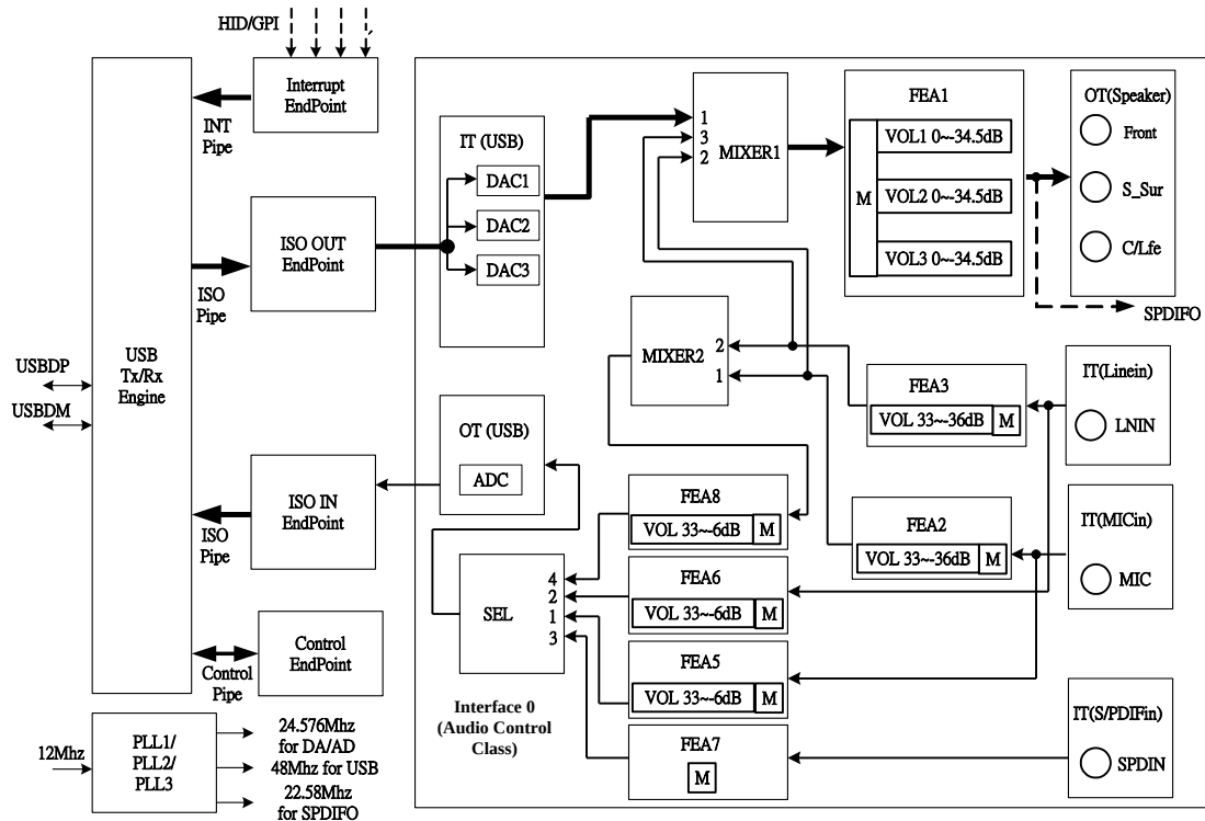
Figure 2 : Function Block Diagram of CM6206LX
