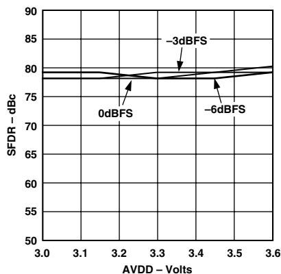
TPC 15. SFDR vs. AVDD @ f_{OUT} = 10 MHz, f_{DAC} = 320 MSPS
