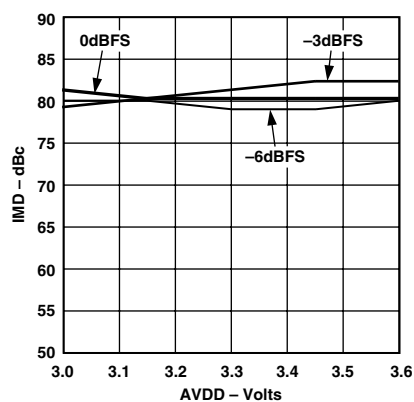
TPC 16. Third Order IMD Products vs. AVDD @ f_{OUT} = 10 MHz, f_{DAC} = 320 MSPS
