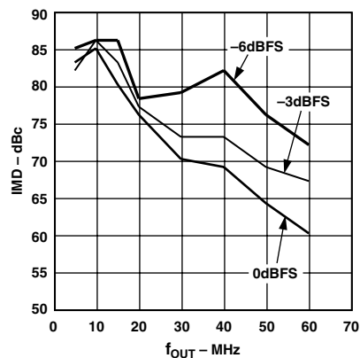
TPC 12. Third Order IMD Products vs. f_{OUT} @ f_{DATA} = 160 MSPS
