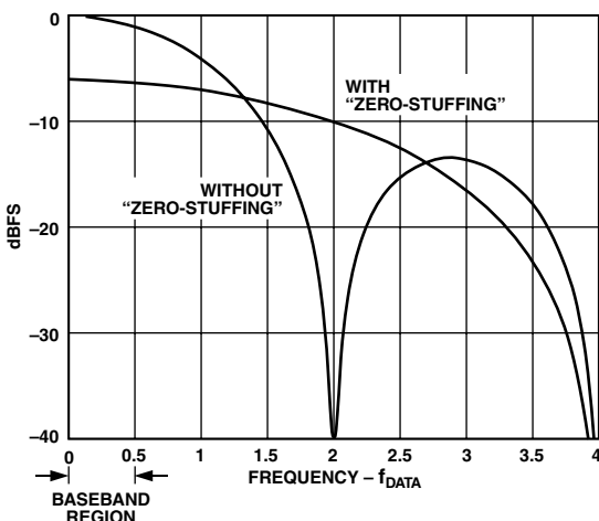
Figure 7. Effects of “Zero-Stuffing” on DAC’s \sin(x)/x Response
