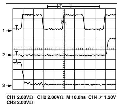
b. Figure 13. RESET Timing of AD9772A with PLL Disabled
