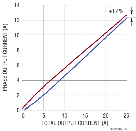
Figure 5. Output Current Sharing ( V_{IN} = 12V , V_{OUT} = 12V )
