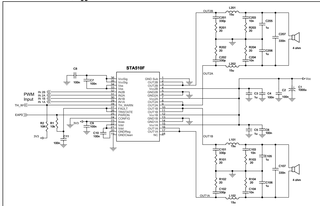
Figure 5. Typical quad half-bridge configuration giving 200 W per channel into 4 \Omega speakers, 10% THD, V_{CC} = 39 V
