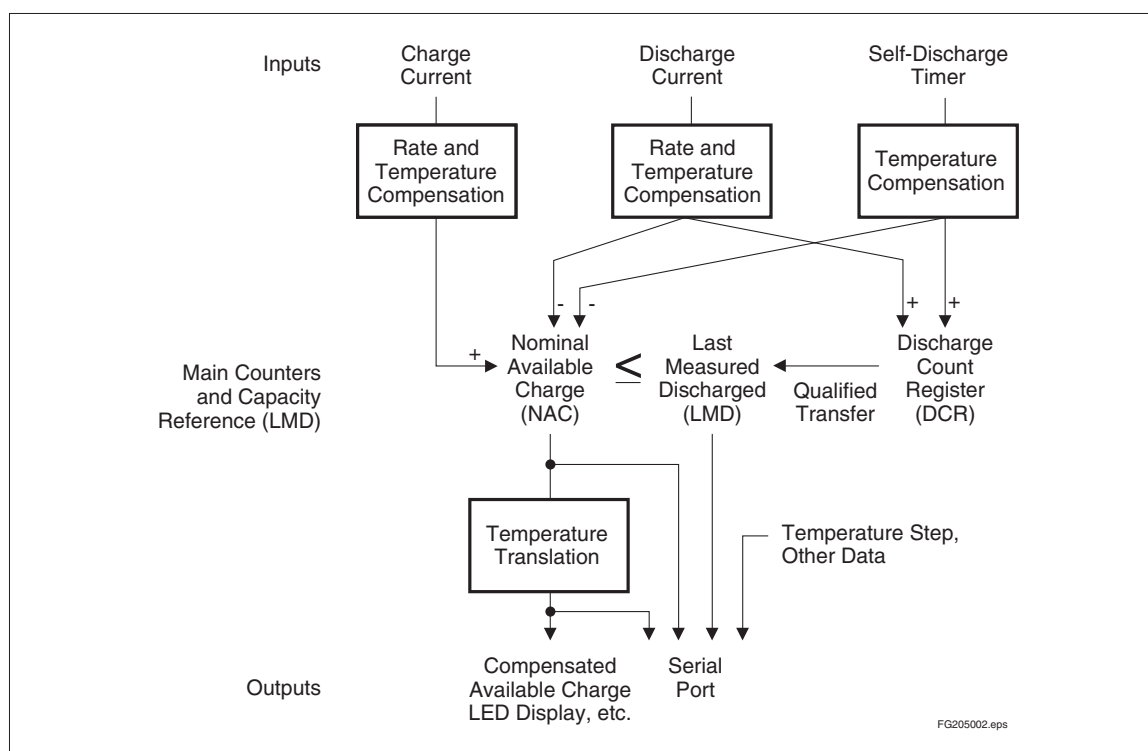
Figure 2. Operational Overview
