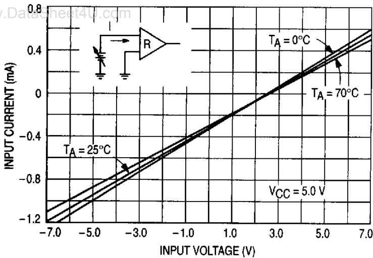
Figure 12. Receiver Input Characteristics
