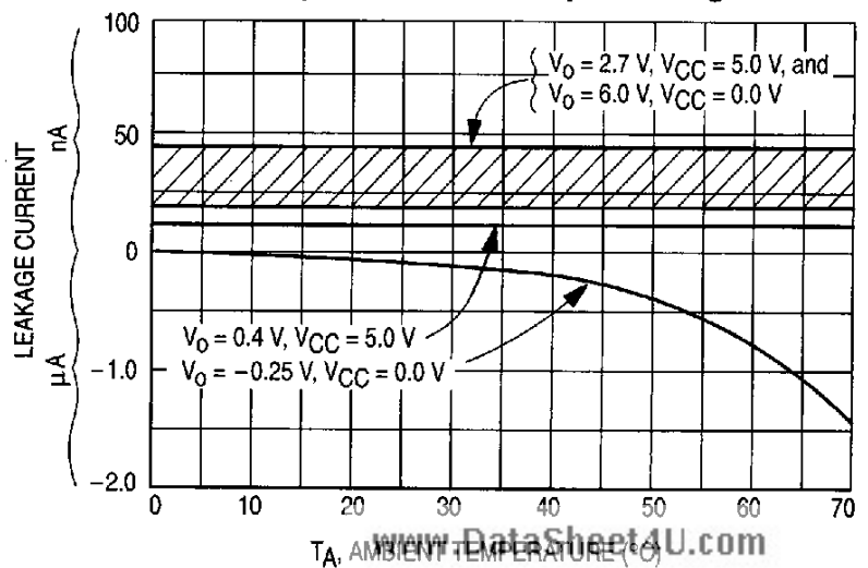
Figure 15. Driver Output Leakage
