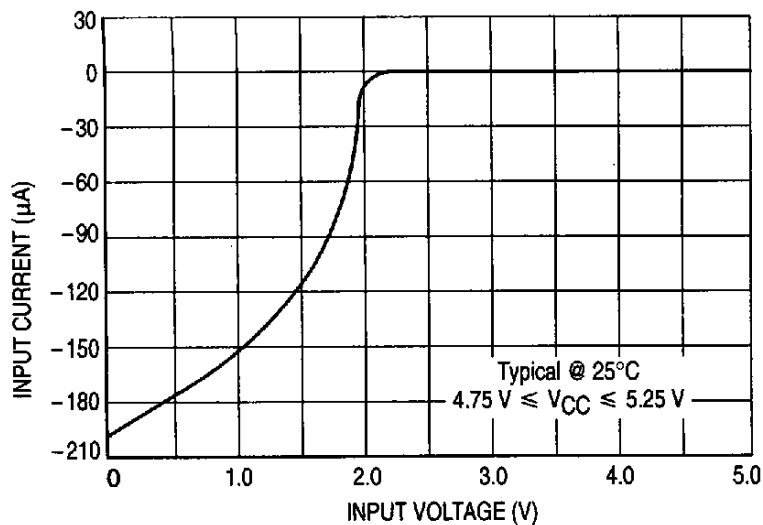
Figure 4. Driver Input Characteristics
