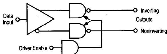
Driver Block Diagram
