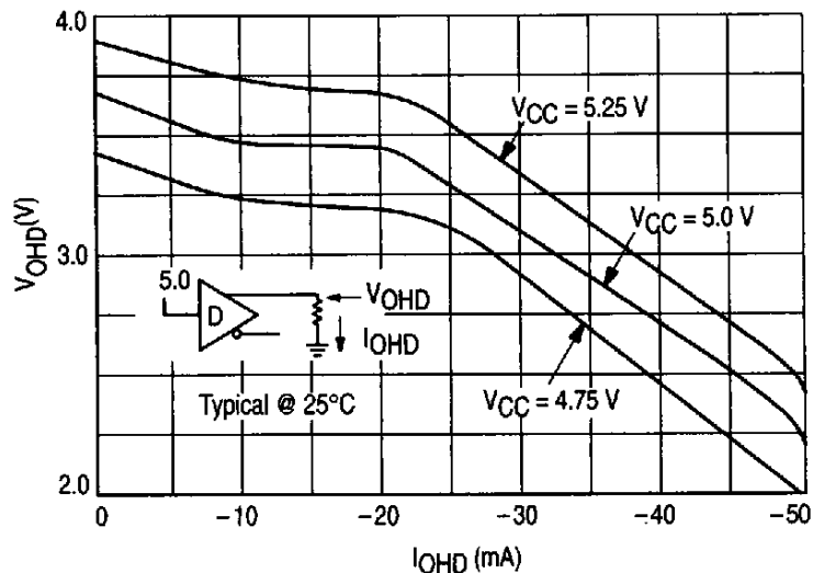
Figure 7. Driver Output Voltage
