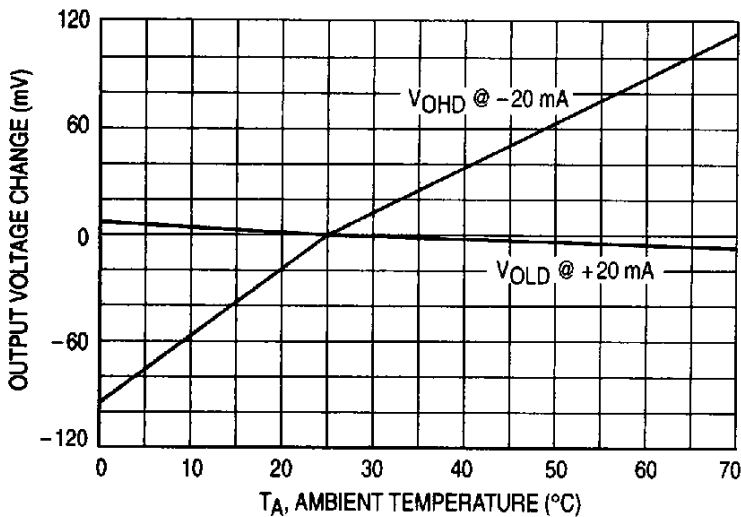
Figure 14. Driver Output Voltage
