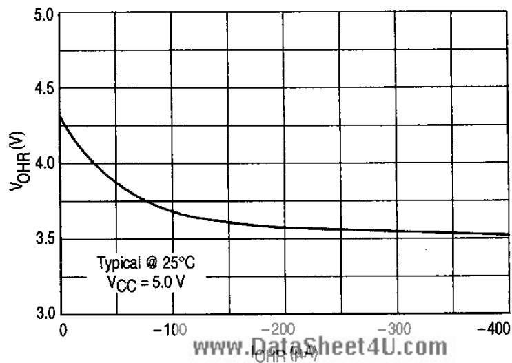
Figure 9. Receiver Output Voltage
