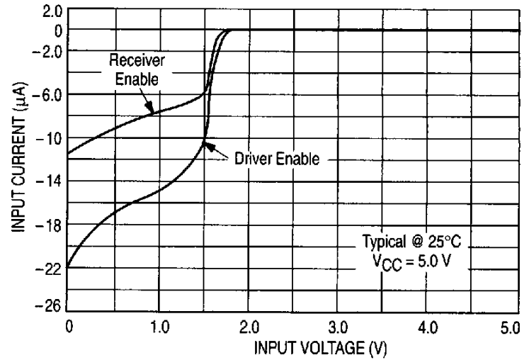
Figure 11. Enable Input Characteristics
