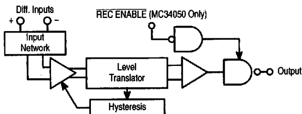
Receiver Block Diagram
