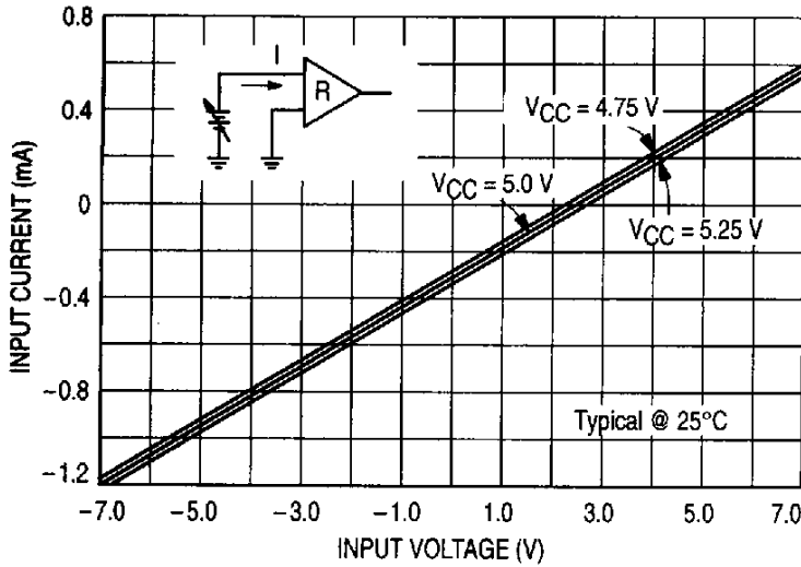
Figure 10. Receiver Input Characteristics
