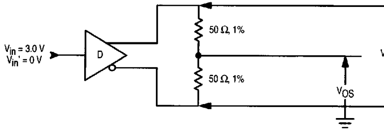
Figure 2. Driver Switching Test Circuits
