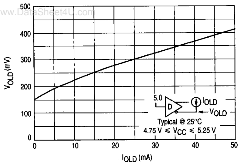
Figure 6. Driver Output Voltage
