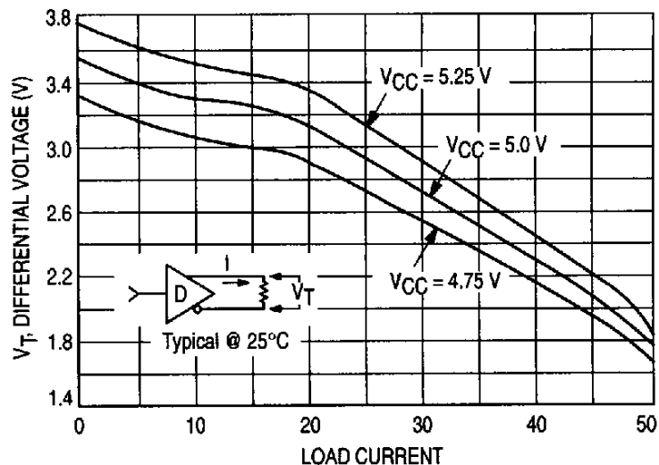
Figure 5. Driver Differential Output Characteristics
