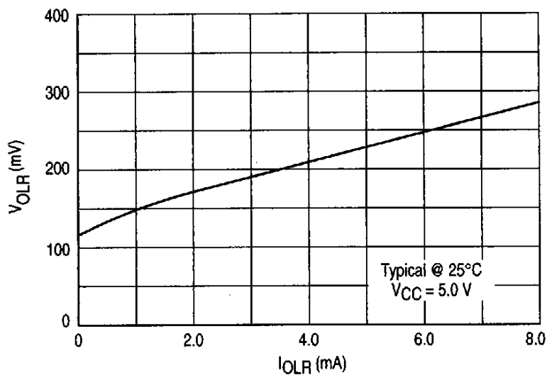
Figure 8. Receiver Output Voltage
