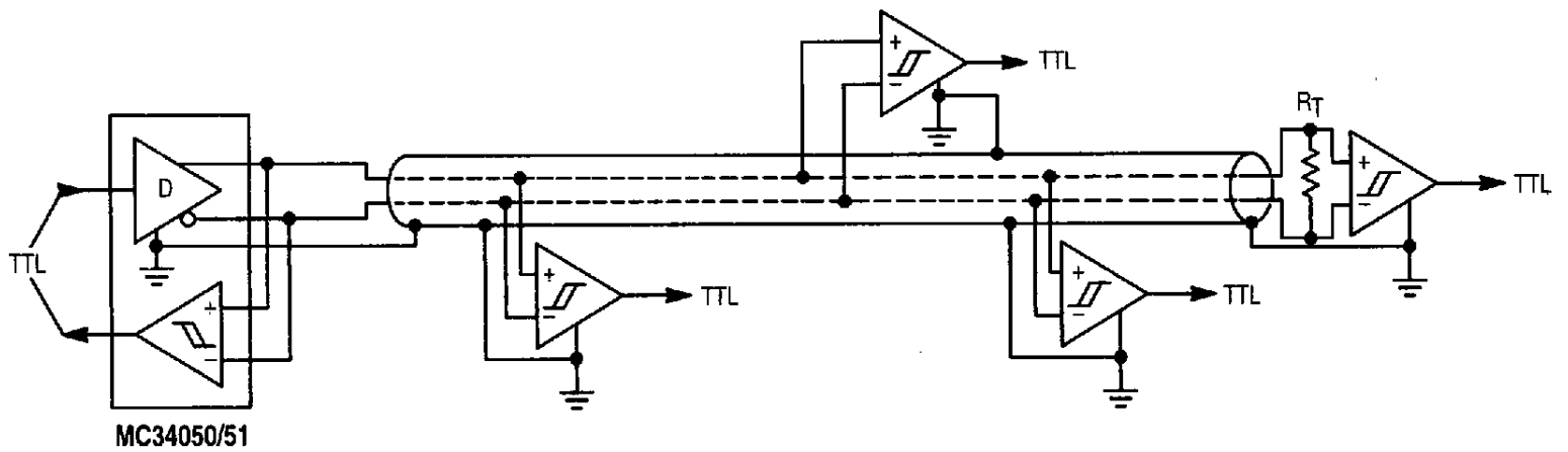
Figure 17. EIA-423 Application
