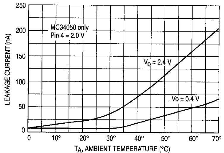
Figure 13. Receiver Output Leakage
