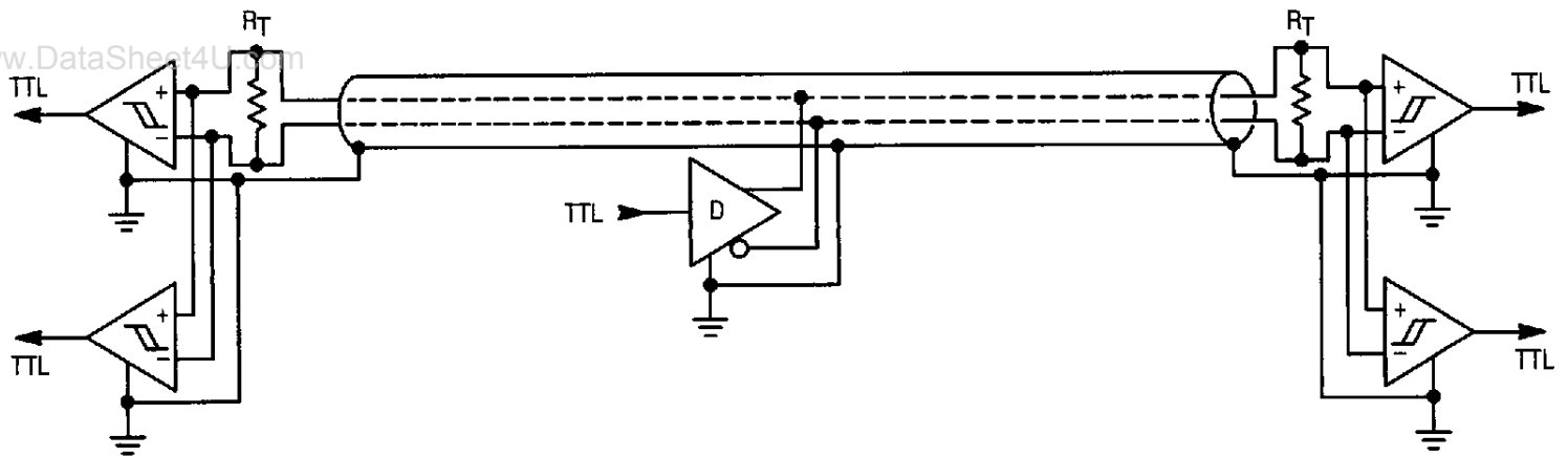
Figure 17. EIA-423 Application
