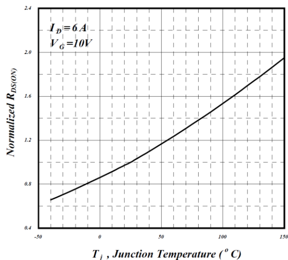
Figure 5.4 Normalized on-resistance v.s. junction temperature
