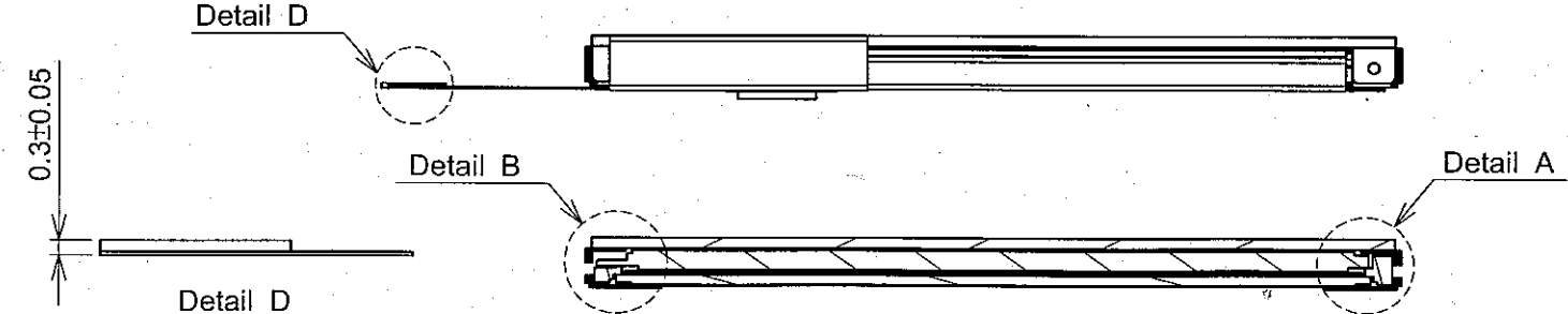
SECTION H2-H2
