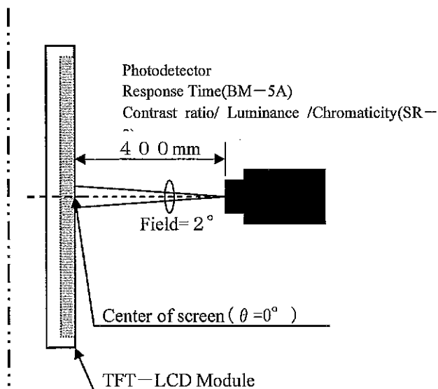
Fig2-2 Luminance/Contrast ratio/Response time/Chromaticity measurement method
