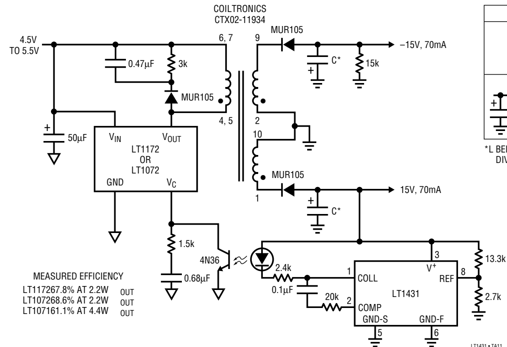
Isolated 5V to ±15V Flyback Converter
