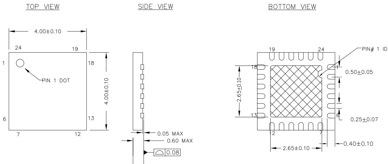
Figure 17. 24-Pin (4 × 4 × 0.55 mm) Sawn QFN
