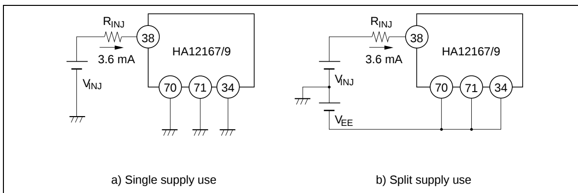
Figure 7 Injector Current Application
