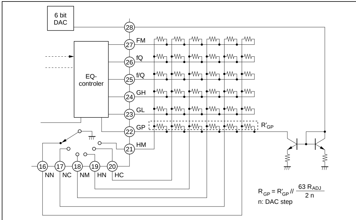
Figure 15 Switch by Tape Select
