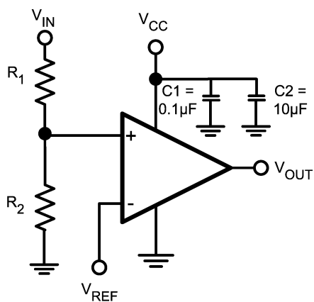
FIGURE 1. Threshold Detector
