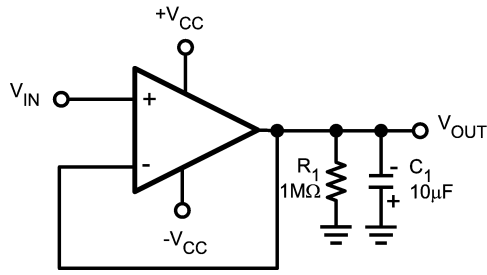
FIGURE 6. Negative Peak Detector
