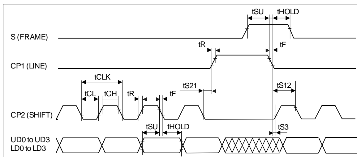
Figure 3. Setup and hold timing diagram
