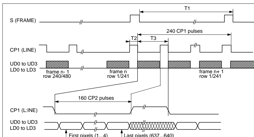
Figure 2. Video input timing diagram
