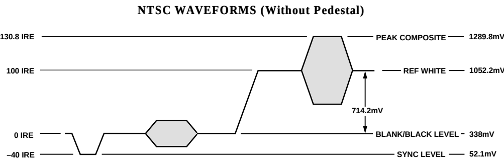
Figure 48. NTSC Composite Video Levels
