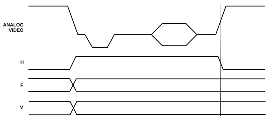
Figure 16. Timing Mode 0 Data Transitions (Master Mode)
