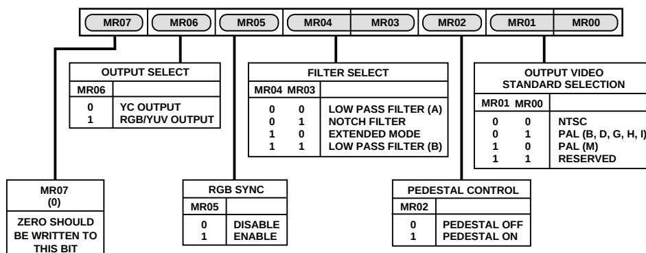
Figure 31. Mode Register 0
