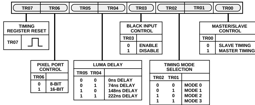
Figure 34. Timing Register 0
