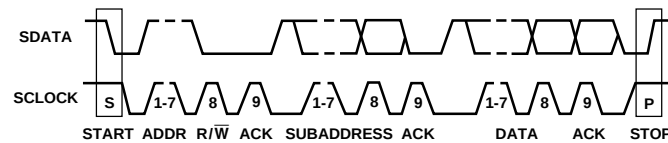
Figure 28. Bus Data Transfer
