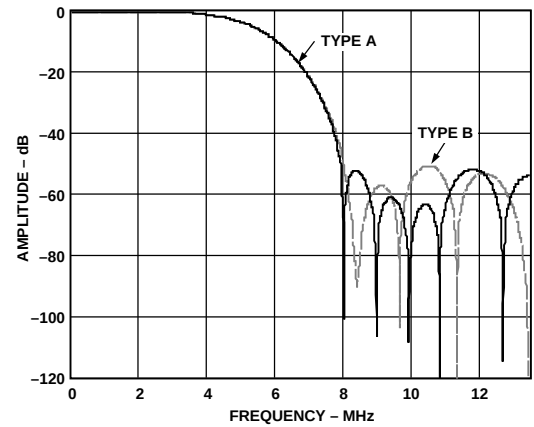
Figure 7. PAL Low-Pass Filter
