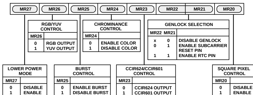
Figure 38. Mode Register 2
