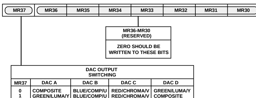
Figure 40. Mode Register 3
