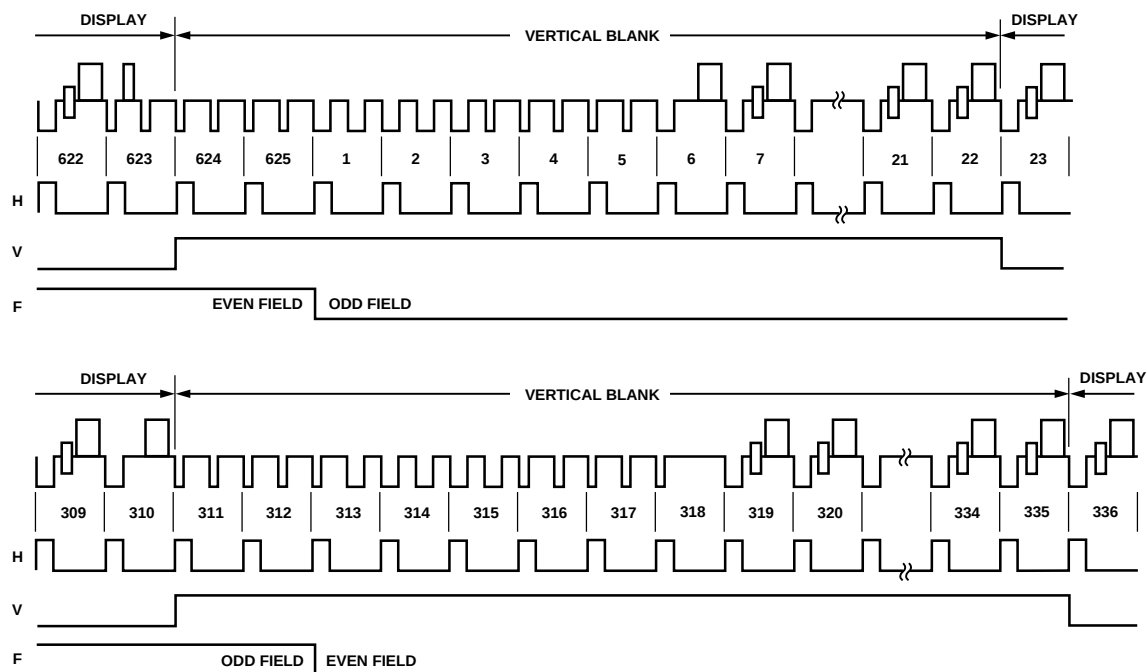
Figure 15. Timing Mode 0 (PAL Master Mode)
