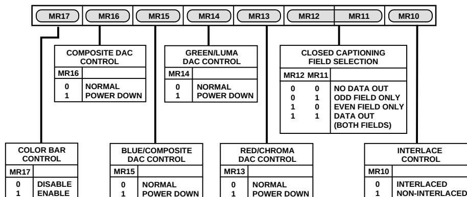
Figure 32. Mode Register 1
