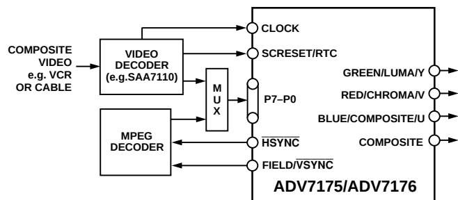
Figure 12. RTC Connections
