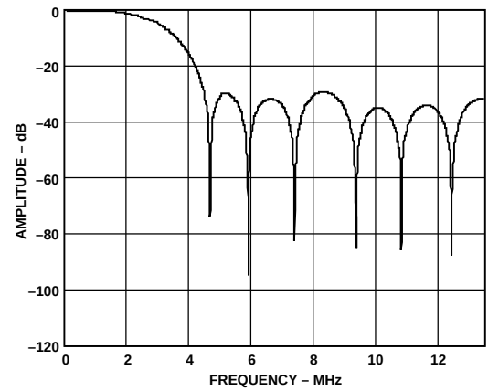
Figure 8. PAL Notch Filter
