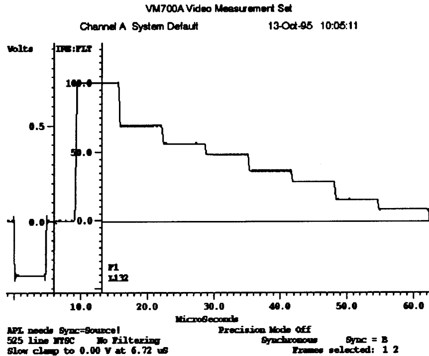
Figure 59. 100/75% Color Bars NTSC (Luminance Only)
