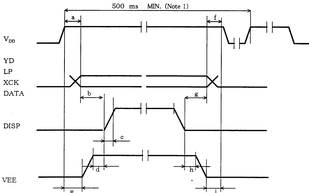
Fig.12 Sequence condition
