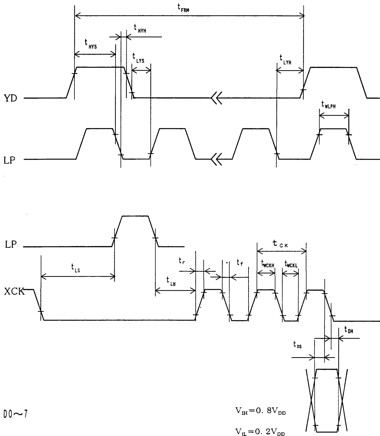
Fig.4 Interface timing chart
