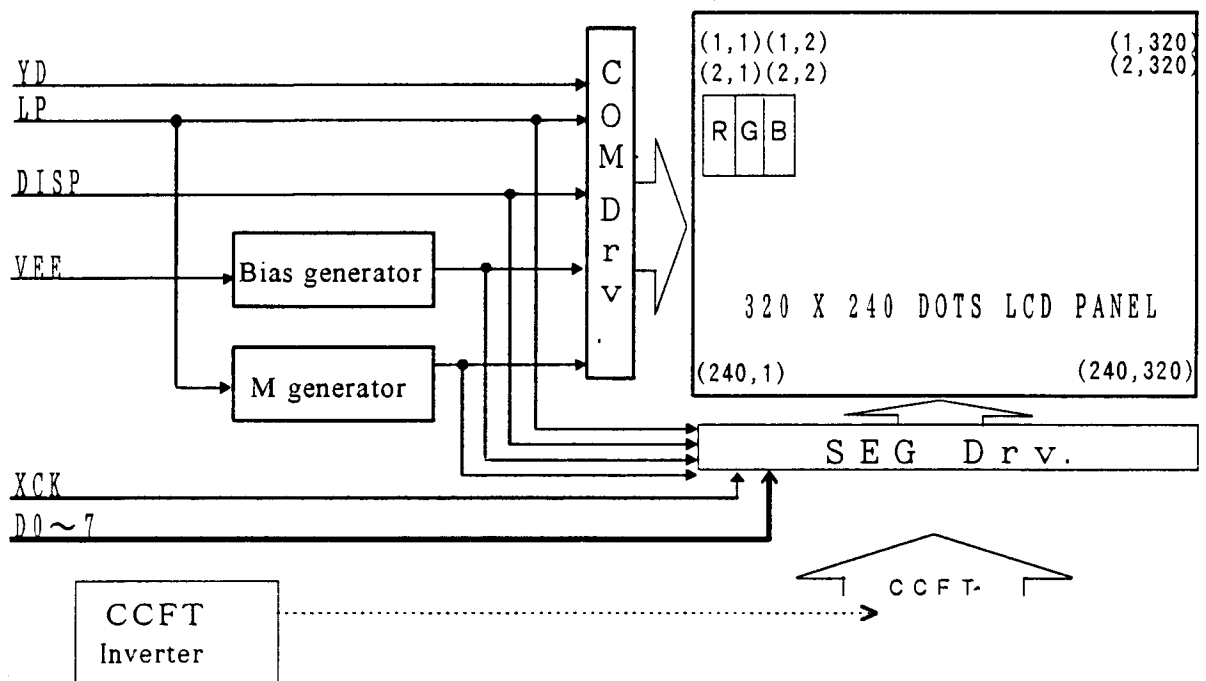
Fig.10 Circuit block diagram
