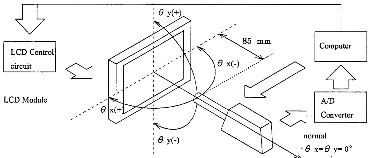
Fig. 8 Optical Characteristics Test Method II
