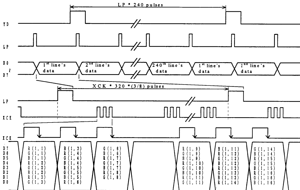
Fig. 2 Interface timing
