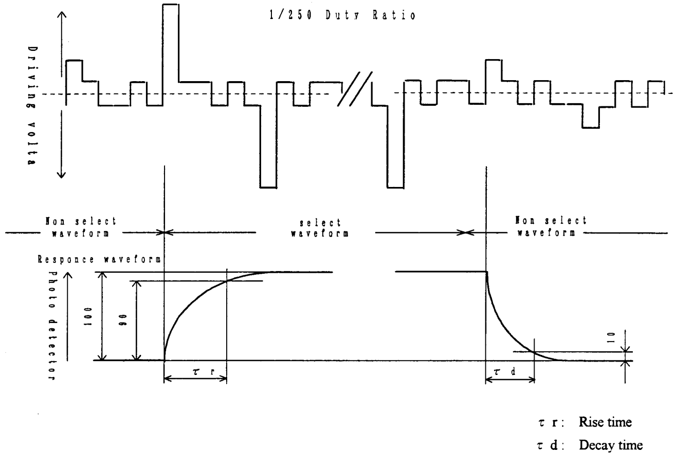
Fig.9 Definition of Response time
