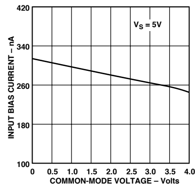
Figure 3. OP462 Input Bias Current vs. Common-Mode Voltage
