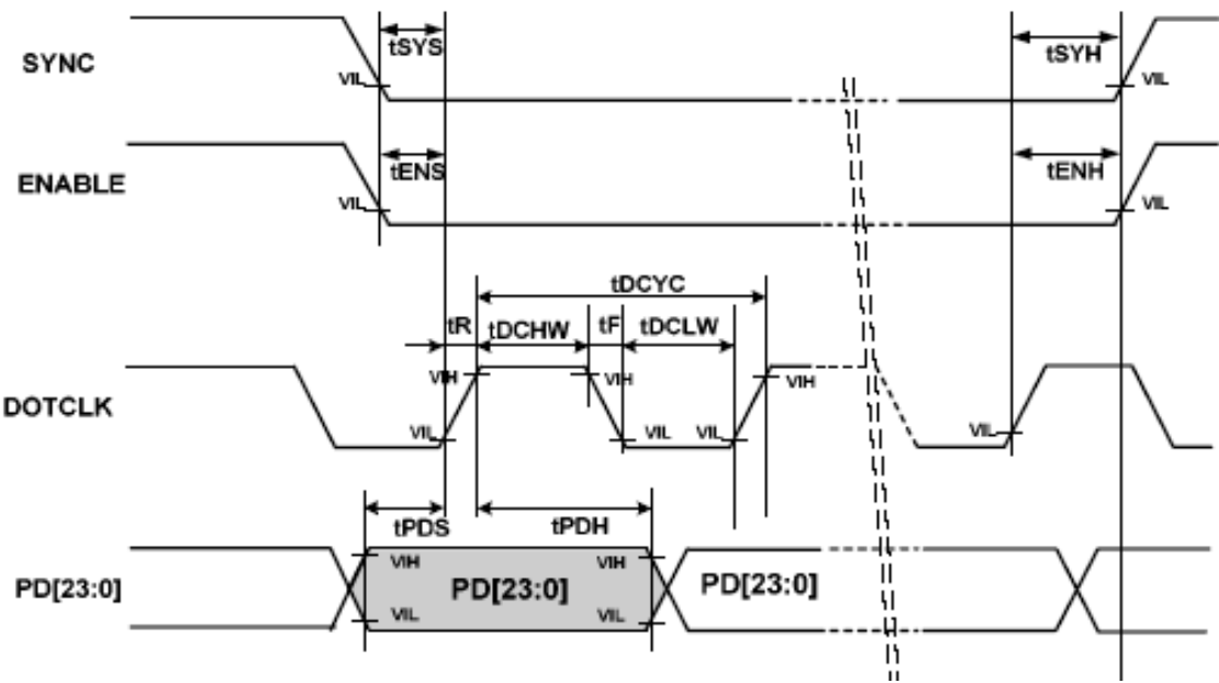
AC Characteristics
