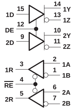
SN65LVDS1050PW (Marked as DL1050 or DLS1050) (TOP VIEW)
