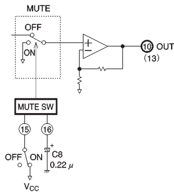
Fig. 10 Mute circuit
