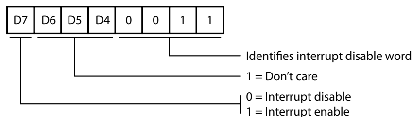
Figure 15. PIO Interrupt Disable Word
