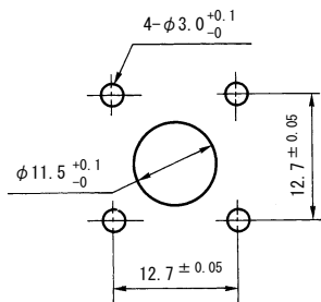
Mounting Hole R
