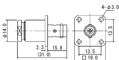
Mounting Hole
