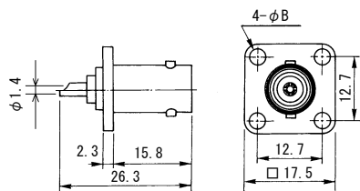
Mounting Hole
