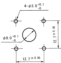
Mounting Hole
