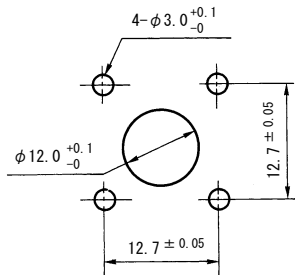
Mounting Hole N
