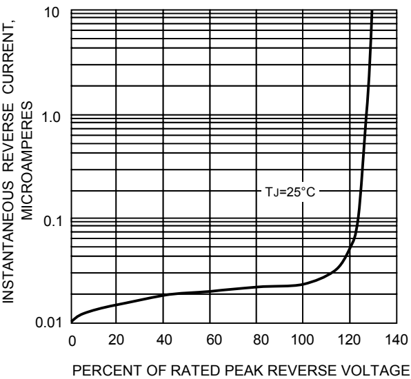
FIG.4-TYPICAL REVERSE CHARACTERISTICS
