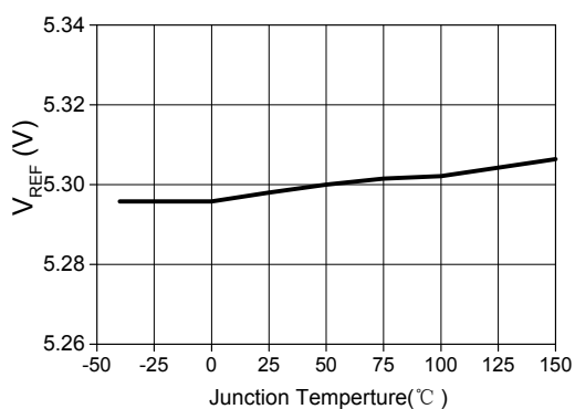
(c) V_{REF} vs T_j
