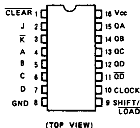
Pin Assignment
