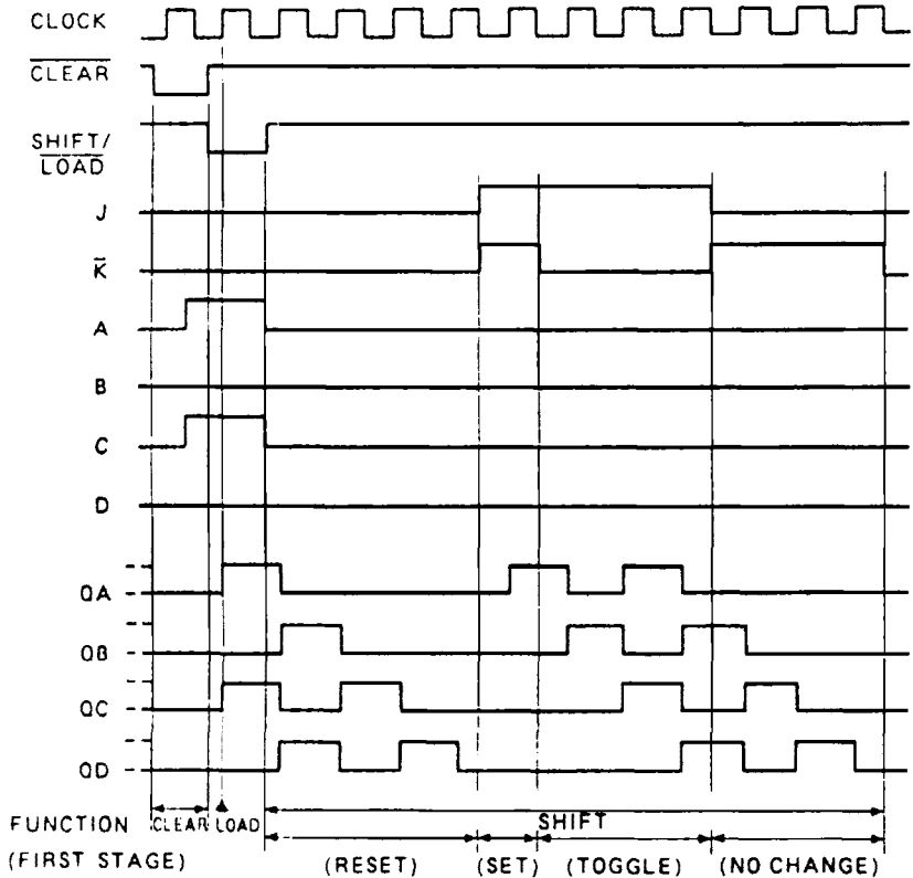
Timing Chart
