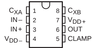
D014, J, OR N PACKAGE (TOP VIEW)
