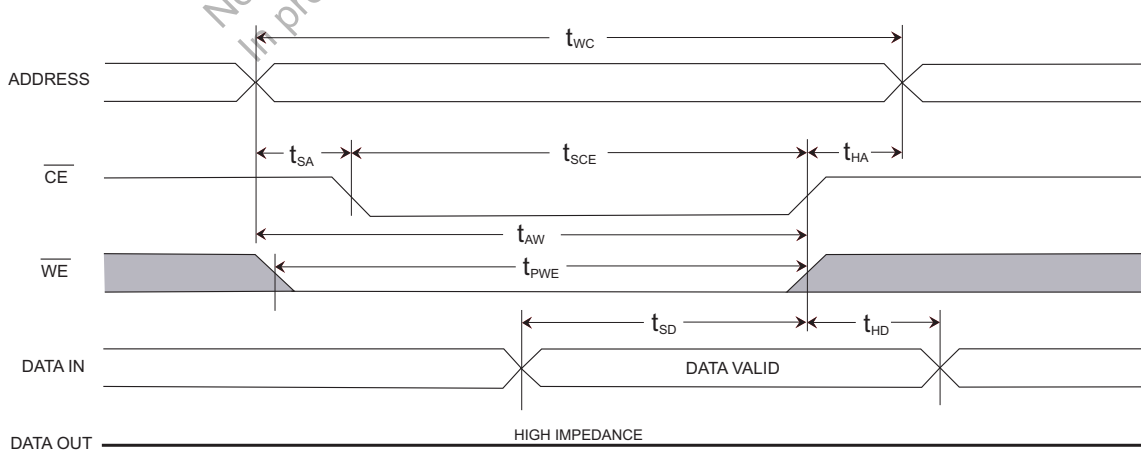
Figure 10. SRAM Write Cycle 2: \overline{CE} Controlled [11, 12]
