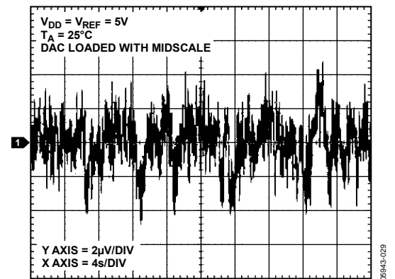
Figure 26. 0.1 Hz to 10 Hz Output Noise Plot
