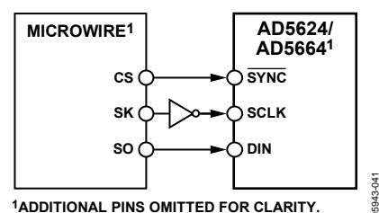
Figure 38. MICROWIRE Interface to AD5624/AD5664
