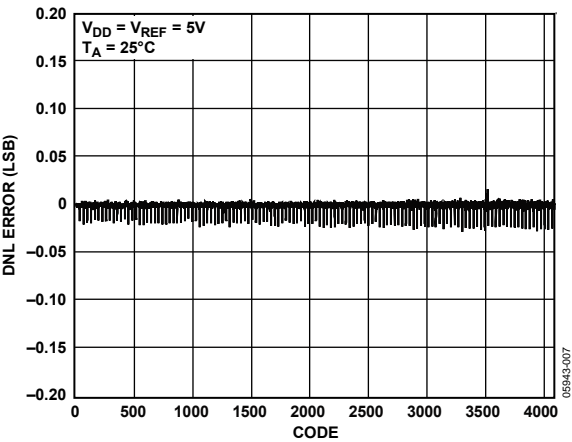
Figure 7. DNL AD5624
