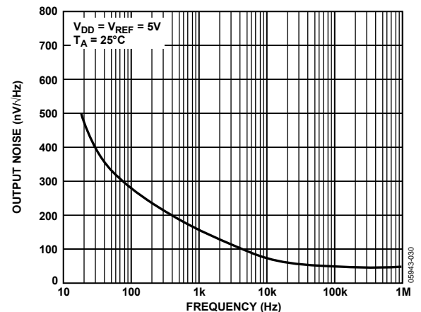
Figure 27. Noise Spectral Density
