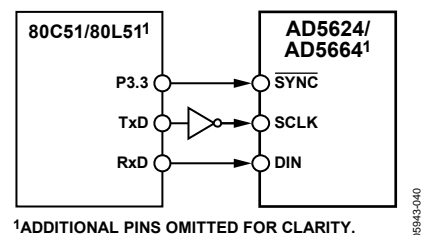
Figure 37. 80C51/80L51 Interface to AD5624/AD5664
