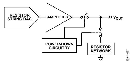
Figure 34. Output Stage During Power-Down
