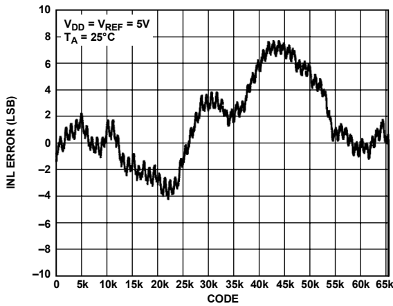
Figure 4. INL AD5664
