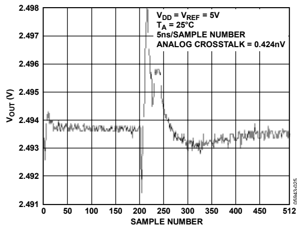
Figure 23. Analog Crosstalk
