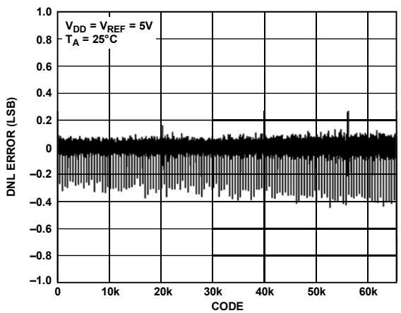
Figure 6. DNL AD5664
