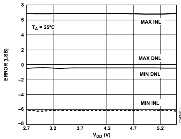
Figure 10. INL and DNL Error vs. Supply
