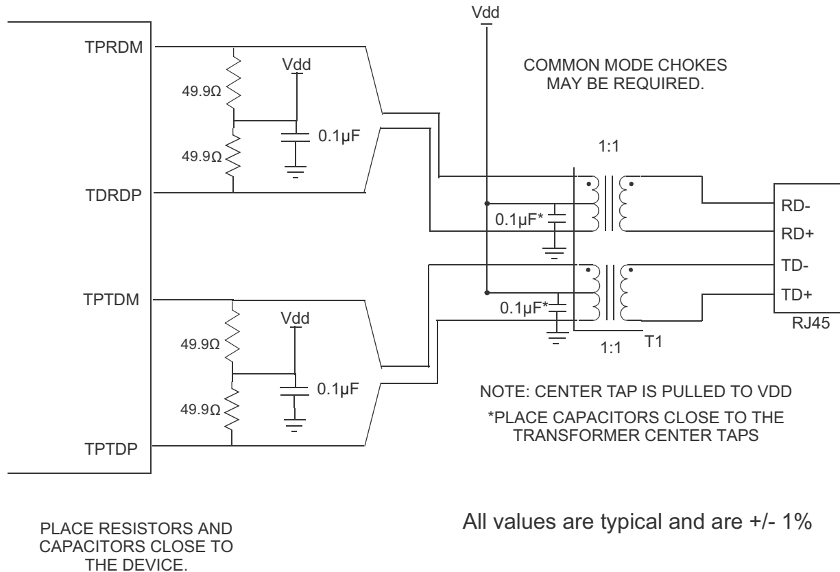
Figure 6-1. 10/100 Mb/s Twisted Pair Interface
