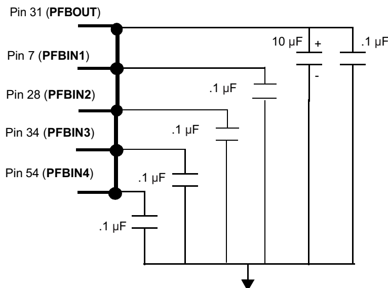
Figure 6-3. Power Feedback Connections
