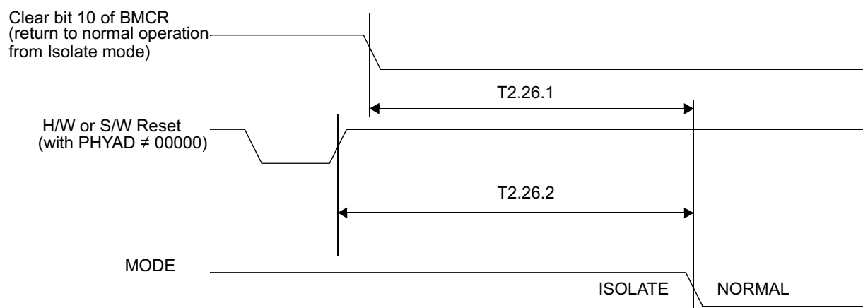
Figure 4-31. Isolation Timing
