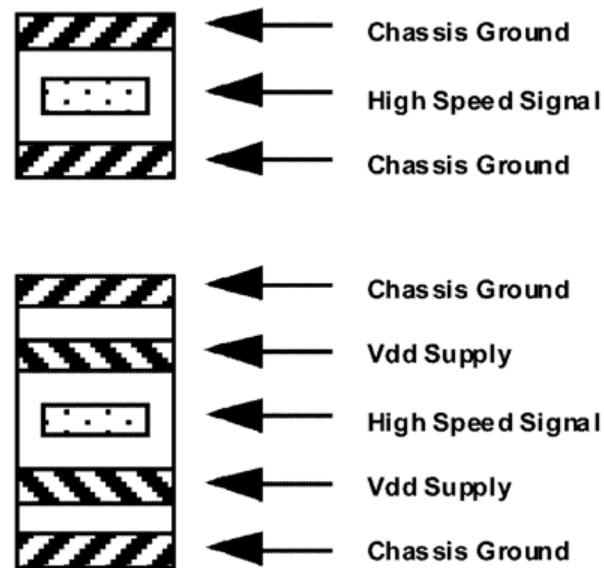
Figure 8-4. Alternative PCB Stripline Layer Stacking
