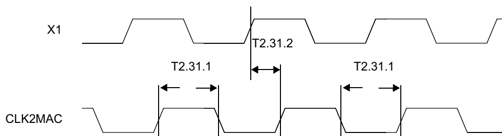
Figure 4-32. CLK2MAC timing
