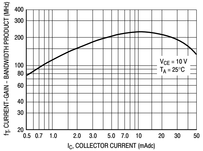
Figure 40. Current-Gain - Bandwidth Product
