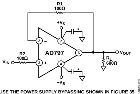
Figure 37. Voltage Follower Connection
