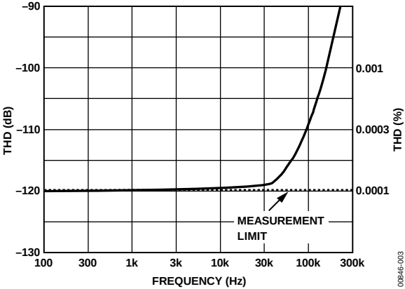
Figure 30. THD vs. Frequency
