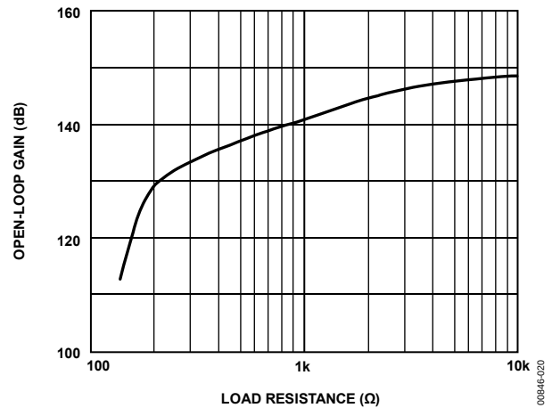
Figure 20. Open-Loop Gain vs. Load Resistance
