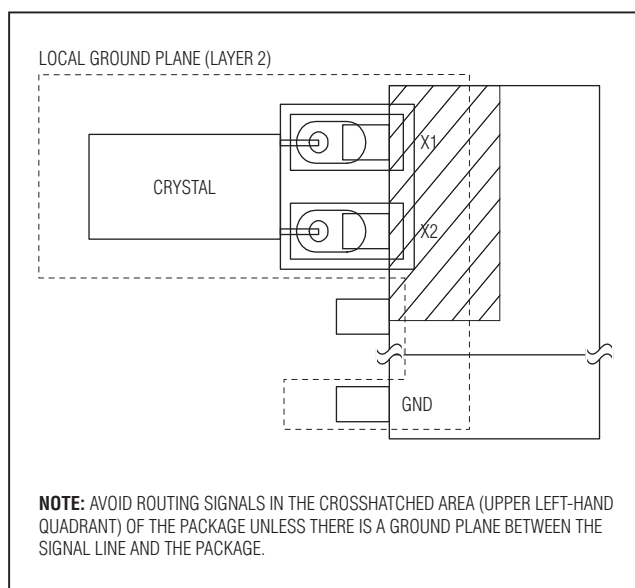
Figure 2. Layout Example
