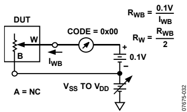
Figure 41. Wiper Resistance
