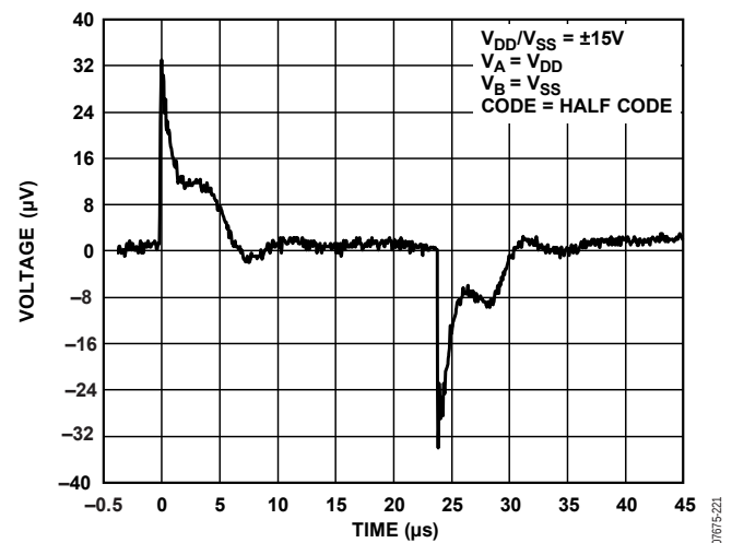
Figure 35. Digital Feedthrough
