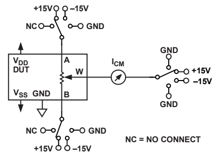
Figure 44. Common-Mode Leakage Current
