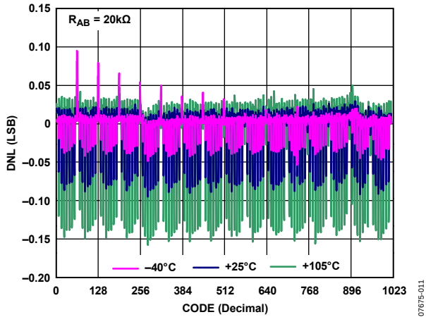
Figure 12. R-DNL in Normal Mode vs. Code vs. Temperature
