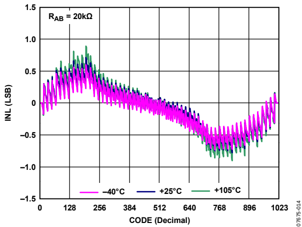
Figure 13. INL in R-Perf Mode vs. Code vs. Temperature
