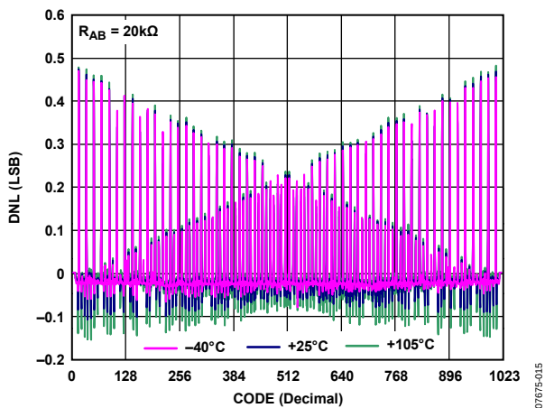
Figure 14. DNL in R-Perf Mode vs. Code vs. Temperature
