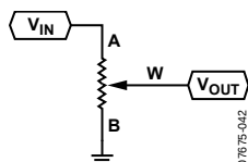
Figure 48. Potentiometer Mode Configuration
