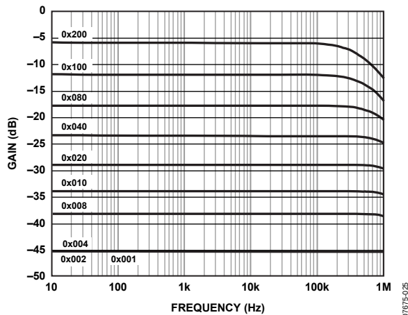
Figure 25. 20 kΩ Gain vs. Frequency vs. Code
