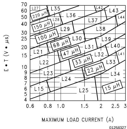
FIGURE 7. LM2596/LM2596HV-ADJ
