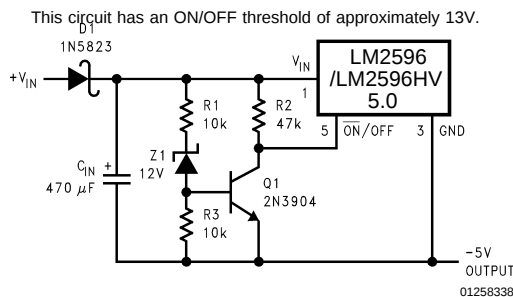
FIGURE 23. Undervoltage Lockout
