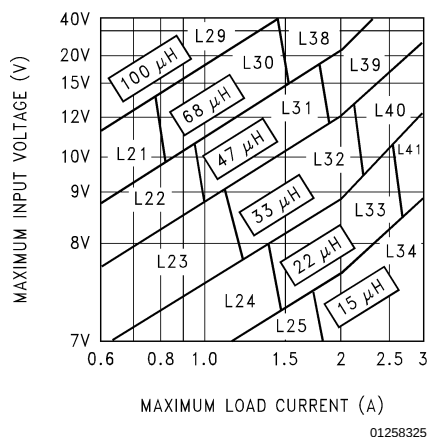
FIGURE 5. LM2596/LM2596HV-5.0
