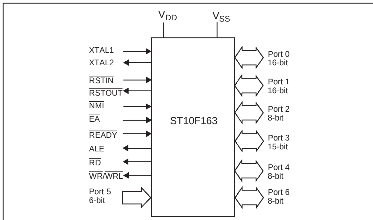
Figure 1 : Logic symbol
