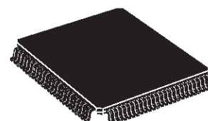
PQFP100 (14 x 14 mm) (Plastic Quad Flat Pack)
