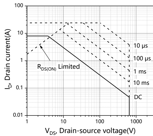
Figure 12. Safe operation area for T_C=25^\circ C
