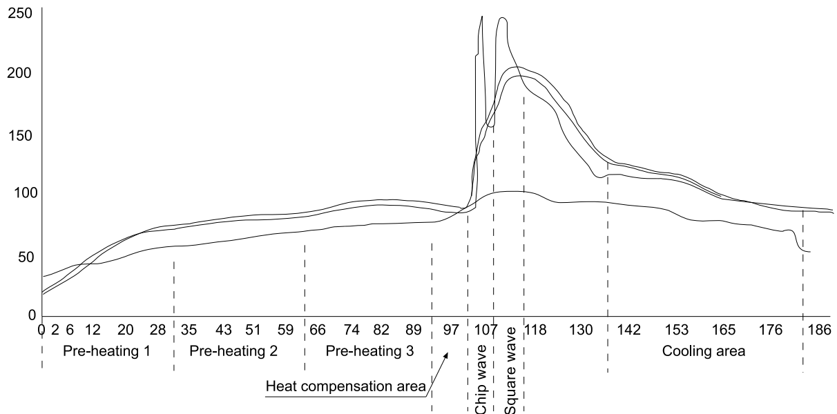
wave soldering temperature distribution chart
