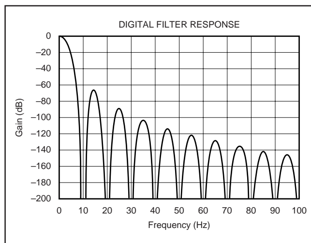
FIGURE 6. Digital Filter Response (10Hz Multiples).
