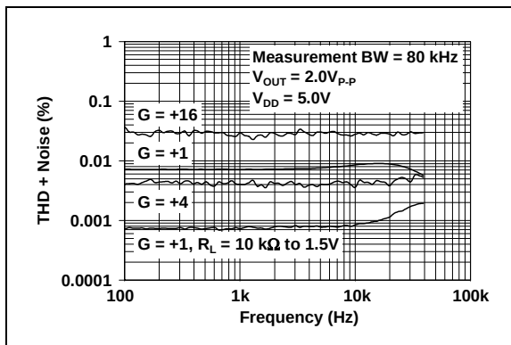
FIGURE 2-27: THD plus Noise vs. Frequency, V_{OUT} = 2 V_{P-P}
