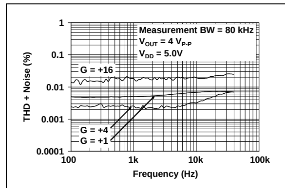
FIGURE 2-30: THD plus Noise vs. Frequency, V_{OUT} = 4 V_{P-P}
