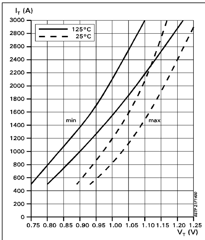
Fig. 2 On-state characteristics.
