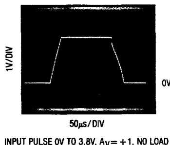
Large Signal Transient Response V S = 5V, 0V
