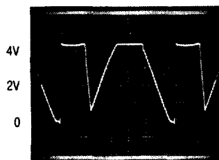
1ms/DIV OP-90 EXHIBITS OUTPUT PHASE REVERSAL
