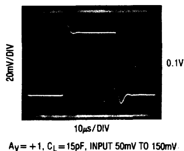
Small Signal Transient Response V S = 5V, 0V
